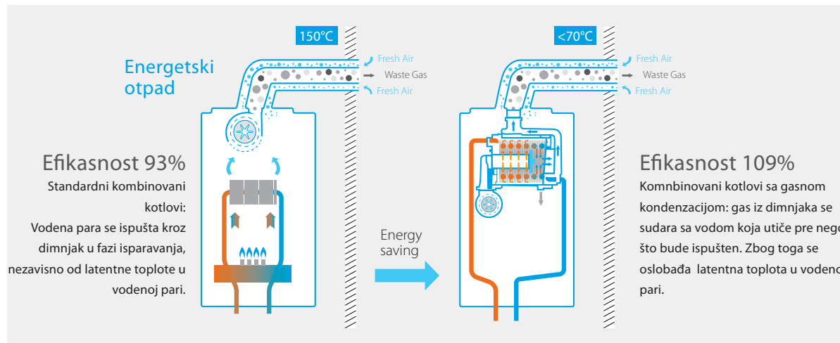
Daikin Altherma C Gas ECH20
